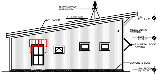
OPTION 1 METAL SIDING
