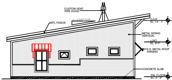
OPTION 2 METAL SIDING METAL WAINSCOTING
