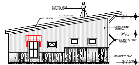
OPTION 3 METAL SIDING STONE WAINSCOTING
